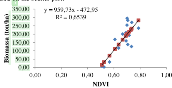
Figure 4. Normality test based on the scatter plot.
